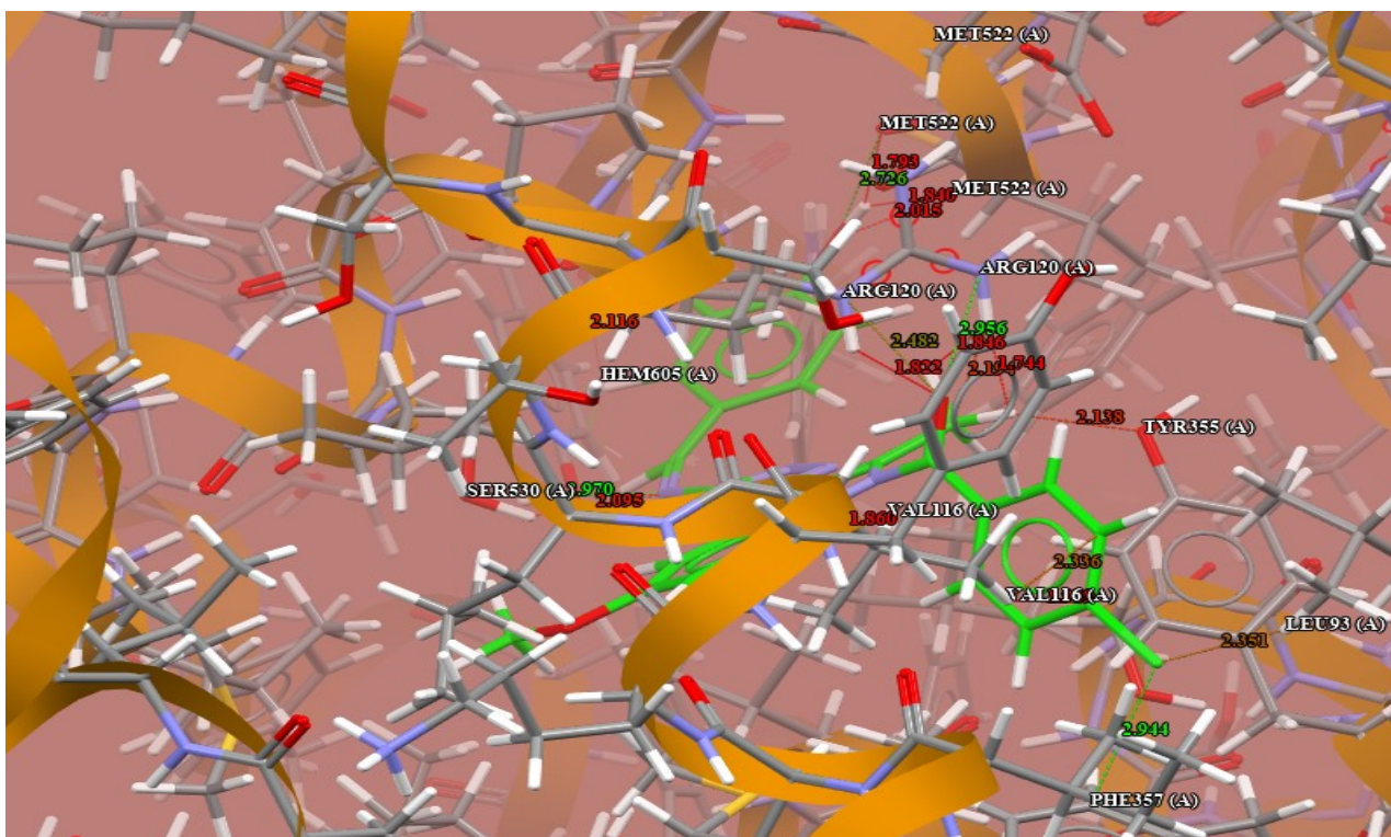
Figure 4. The interaction profile of compound [S2] with the COX2 receptor is characterized by H-bonds and short contacts (PDB code: 4m11). The interaction of substance [S4] with amino acid residues through H-bond [Arg120(2), MET522, SER530, PHE357] is represented in green, whereas short contact is represented in red. [S2: ball and stick, with amino acids in capped sticks]
