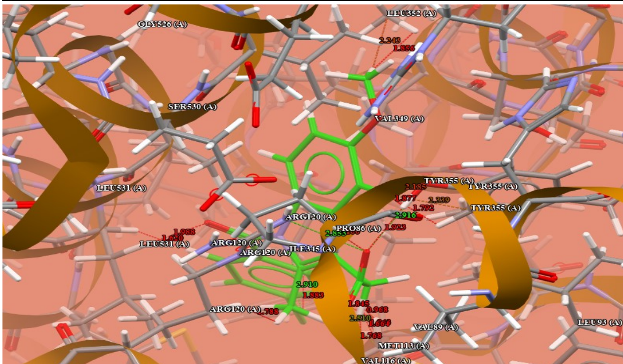
Figure 3. The standard drug Indomethacin's H-bond and short contact interaction profile with the COX2 receptor (PDB code: 4m11). The interaction of Indomethacin with amino acid residues through H-bond [Arg120, TYR355] is represented in green, whereas the short contact is represented in red. [Indomethacin is shown in a ball and stick fashion, whereas amino acids are shown as capped sticks.]
