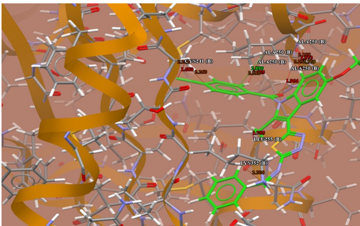
Figure 10. The interaction profile of compound [S5] with the TPI receptor includes H-bonds and short contacts (PDB code: 1SA0). The connection between compound [S5] and amino acid residues via H-bond [ALA250] is represented in green, whereas short contact is represented in red. [S5: ball and stick, with amino acids in capped sticks]
