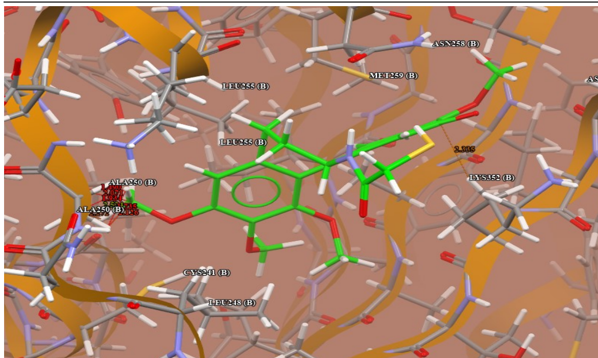
Figure 7. The standard medication Colchicine's H-bond and short contact interaction profile with the TPI receptor (PDB code: 1SA0). The connection between Colchicine and amino acid residues via H-bond [ALA250] is represented in green, whereas short contact is represented in red. [Colchicine is shown in a ball-and-stick fashion, whereas amino acids are shown in capped sticks]
