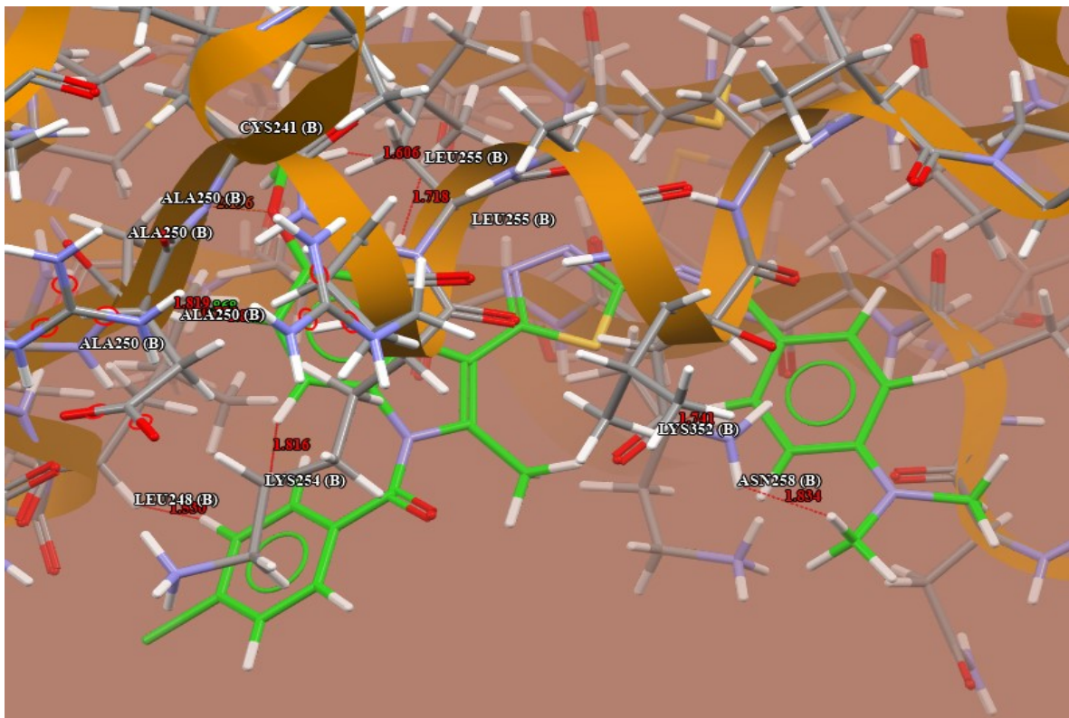
Figure 9. The interaction profile of compound [S4] with the TPI receptor includes H-bonds and short contacts (PDB code: 1SA0). The connection between compound [S4] and amino acid residues via H-bond [ALA250] is represented in green, whereas short contact is represented in red. [S4: ball and stick, with amino acids in capped sticks]
