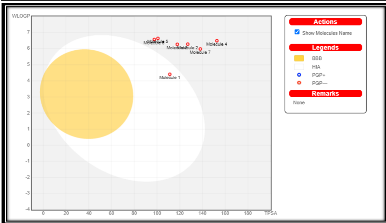
Figure 1. BOILED-EGG for the designed compounds
