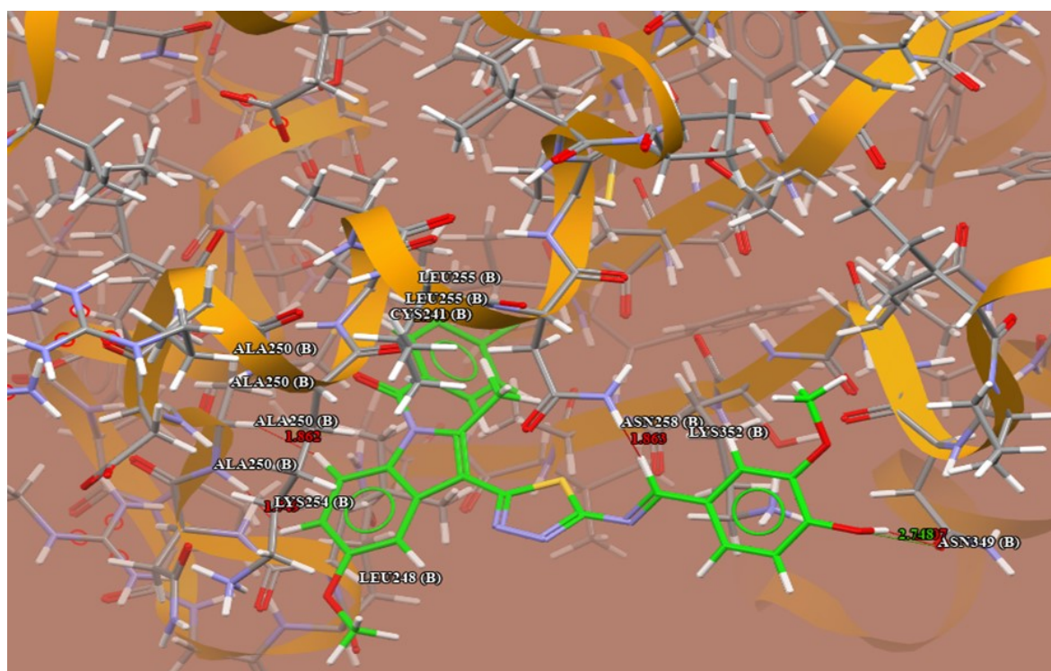
Figure 8. Compound [S1] H-bond and short contact interaction profile with TPI receptor (PDB code: 1SA0). The connection between compound [S1] and amino acid residues via H-bond [ASN349] is represented in green, whereas short contact is represented in red. [S1: ball and stick, with amino acids in capped sticks]
