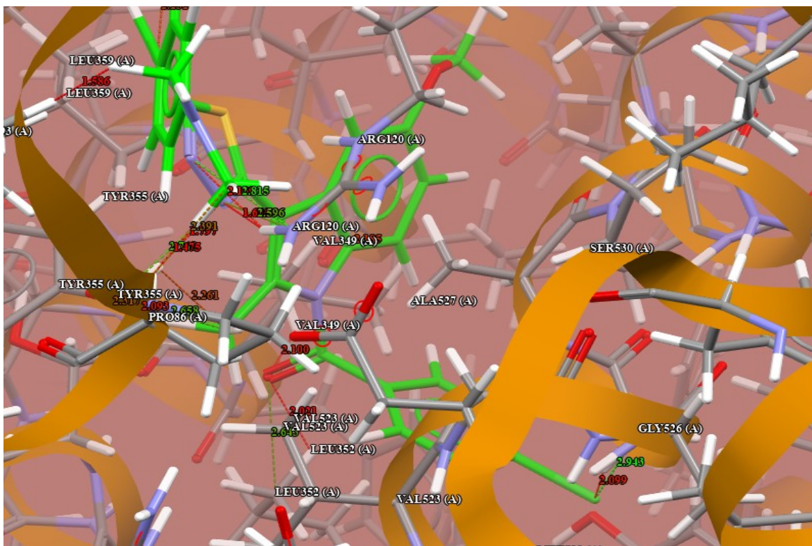
Figure 6. The interaction profile of compound [S6] with the COX2 receptor includes H-bonds and short contacts (PDB code: 4M11). The connection between compound [S6] and amino acid residues via H-bond [GLY526] is represented in green, whereas short contact is represented in red. [S6: ball and stick, with amino acids in capped sticks]
