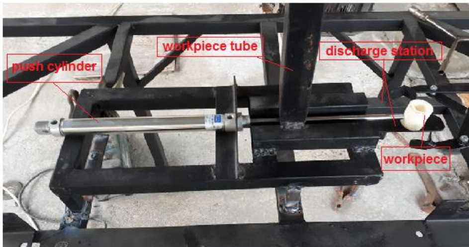
Figure 3 feeding unit
