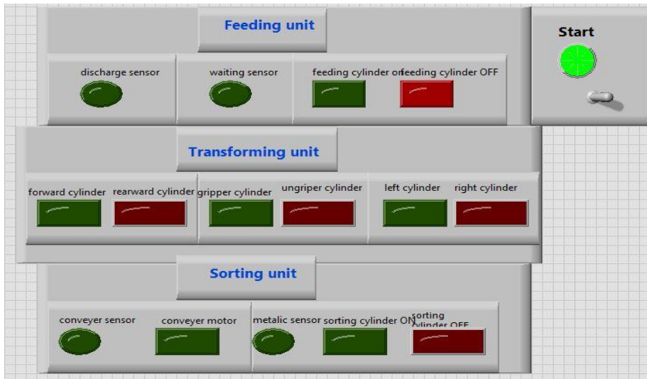
Figure (7) the front panel to monitor the system (HMI for SCADA)
