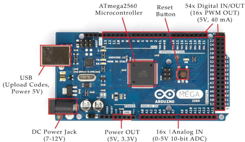
Figure (2)Arduino mega 2560[6]
