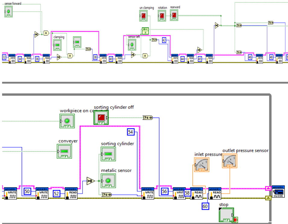
Figure (6) the block diagram of control the system
