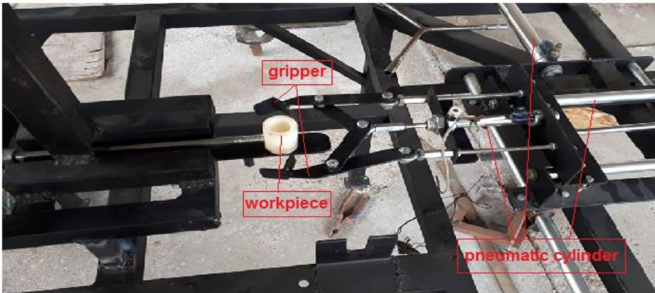
Figure 4 Transporting unit
